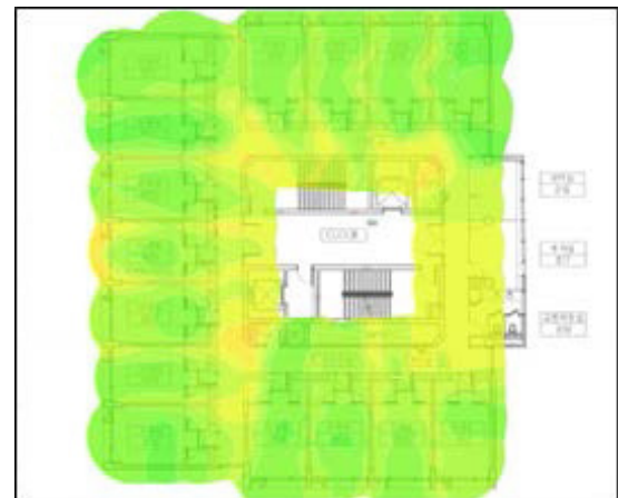
5GHz Wi-Fi Signal Strength on the 8th Floor
